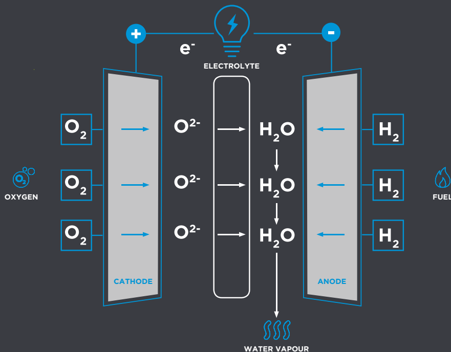
Fig. Principle of a fuel cell
